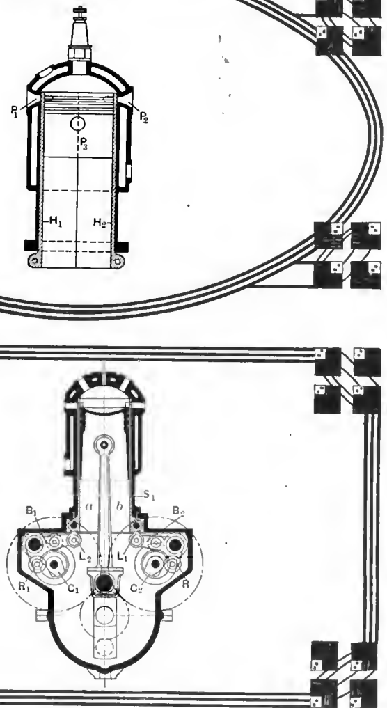
Fig. I—Transverse sectional view of the Redrup motor in which two hemispherical sleeves cover and uncover the valve ports
